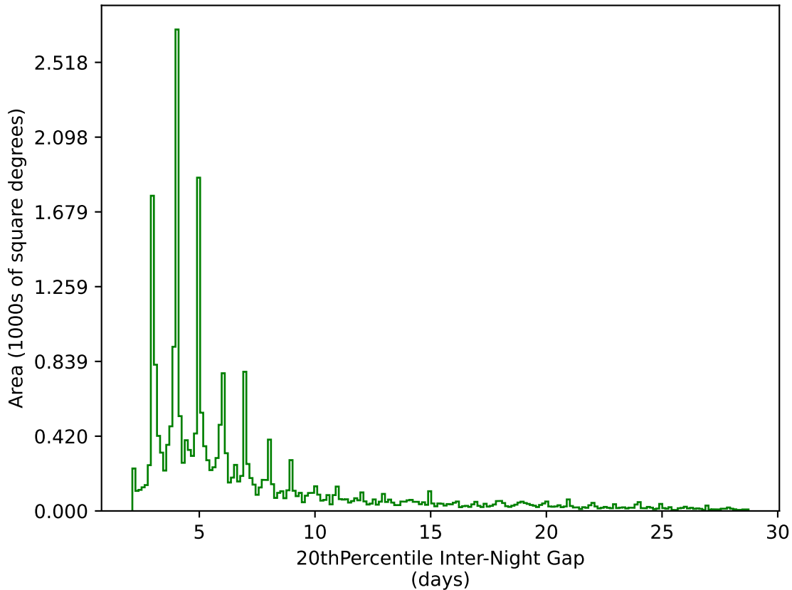
too_100_4v3.4_10yrs All sky g band: 20thPercentile Inter-Night Gap
