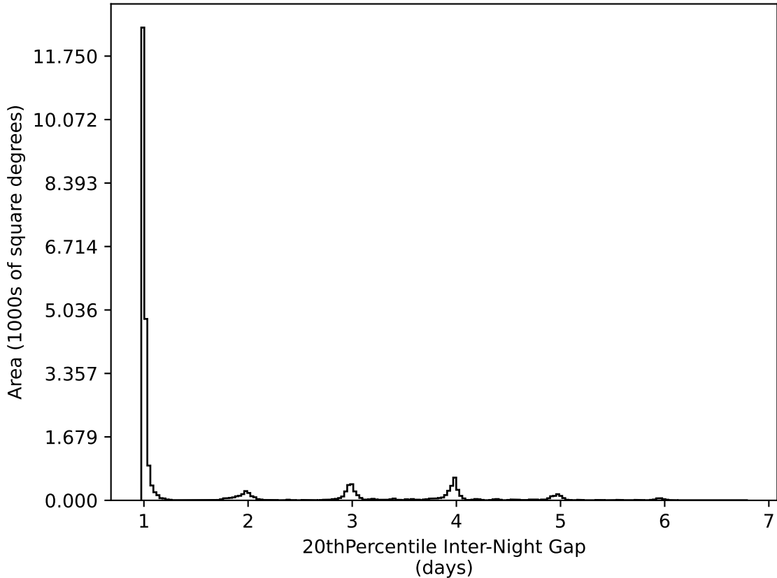
too_100_4v3.4_10yrs All sky all bands: 20thPercentile Inter-Night Gap
