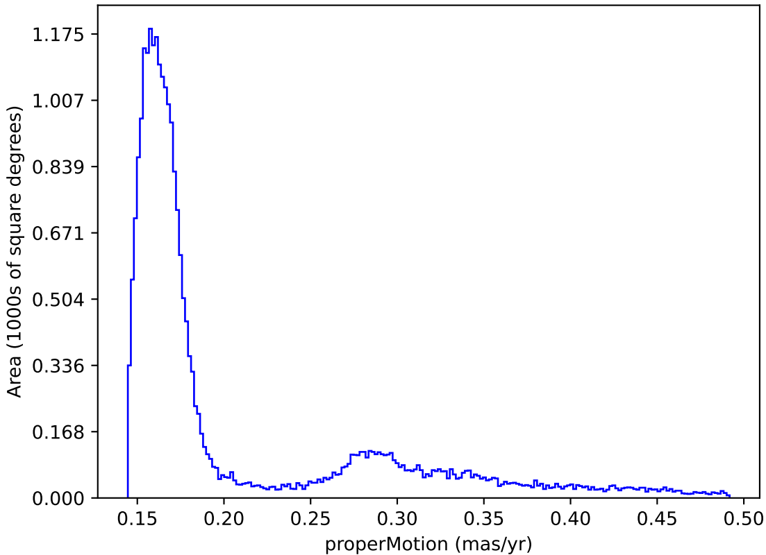
too_100_4v3.4_10yrs : properMotion
