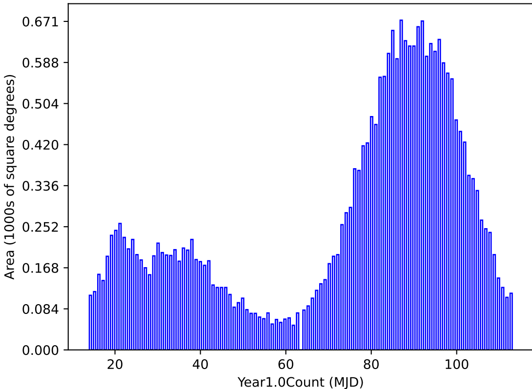
too_100_4v3.4_10yrs night < 365.25: Year1.0Count
