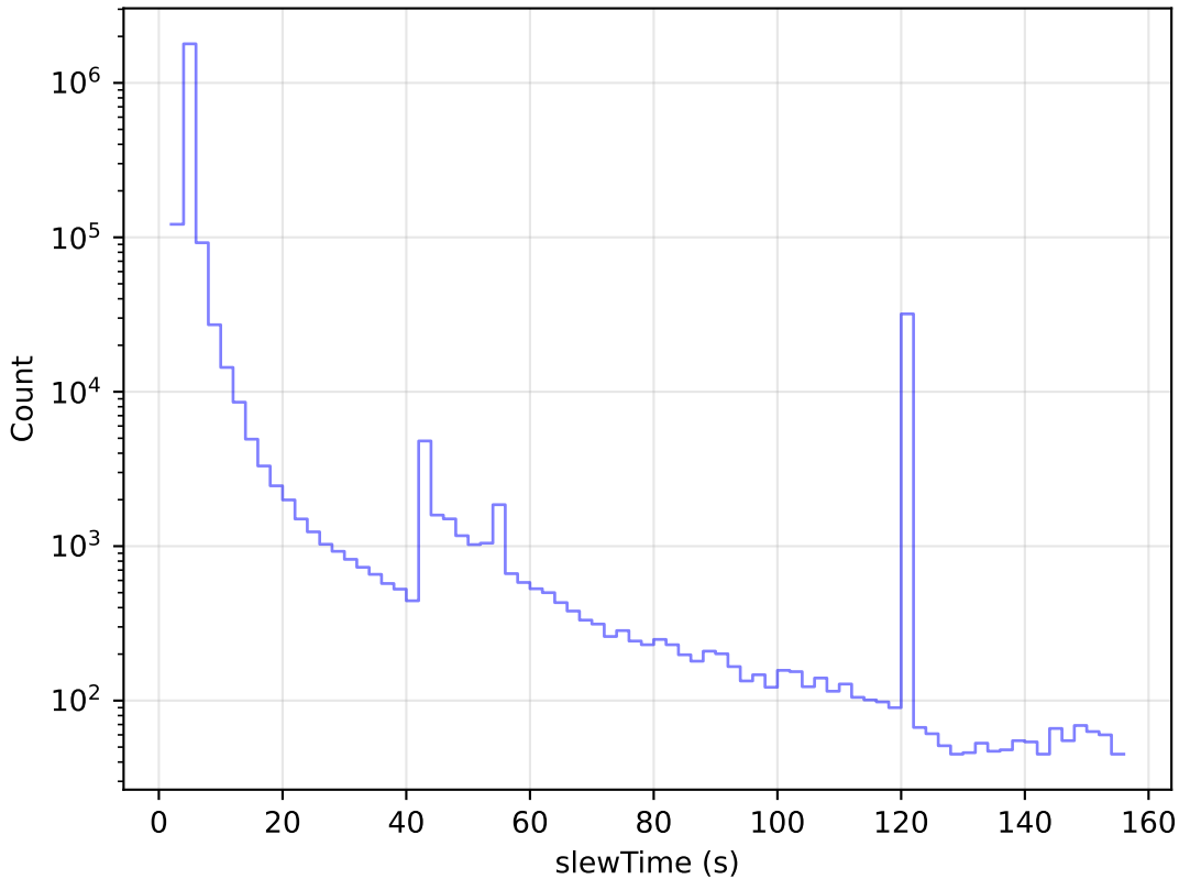
too_100_4v3.4_10yrs All visits: Slew Time Histogram
