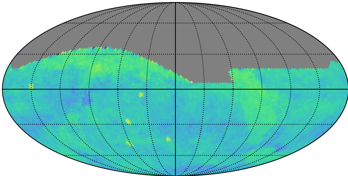
too_100_4v3.4_10yrs (g or r or i): PairFraction
