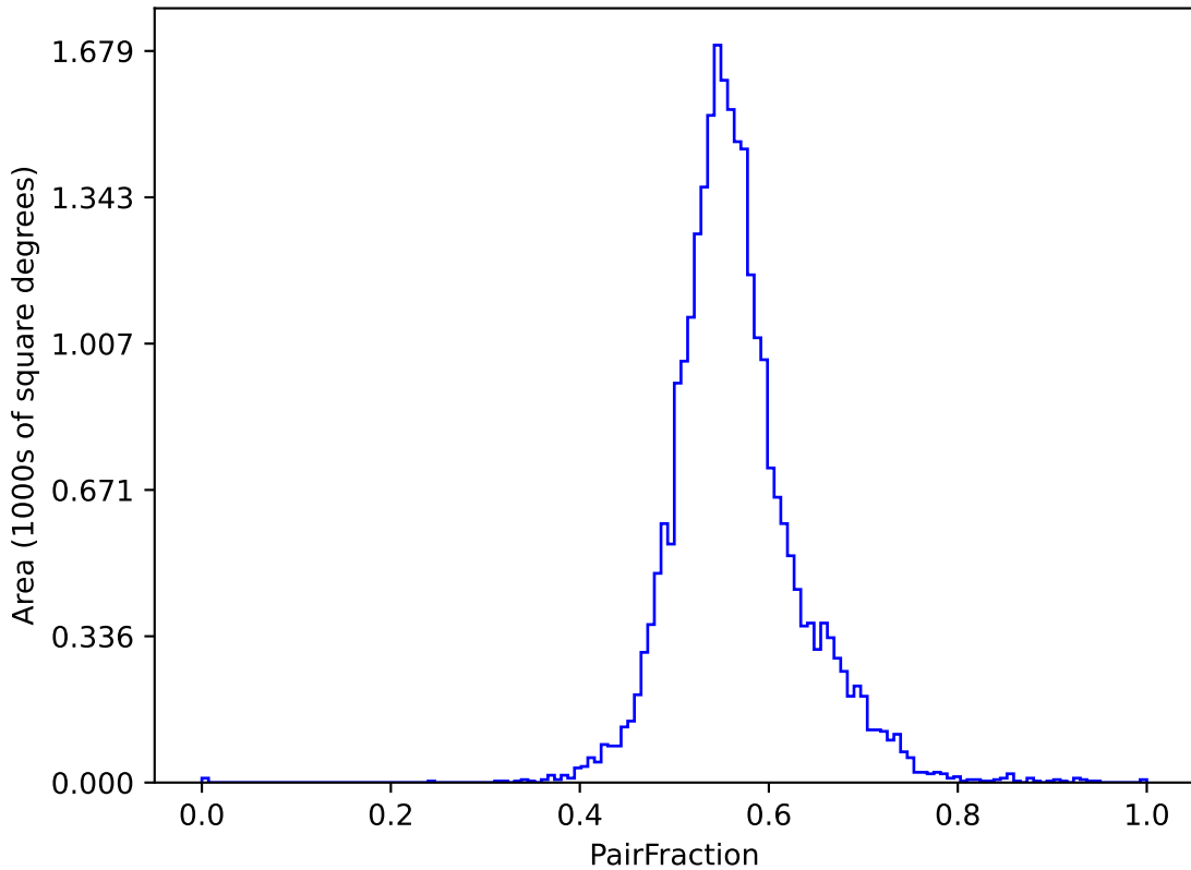
too_100_4v3.4_10yrs (g or r or i): PairFraction
