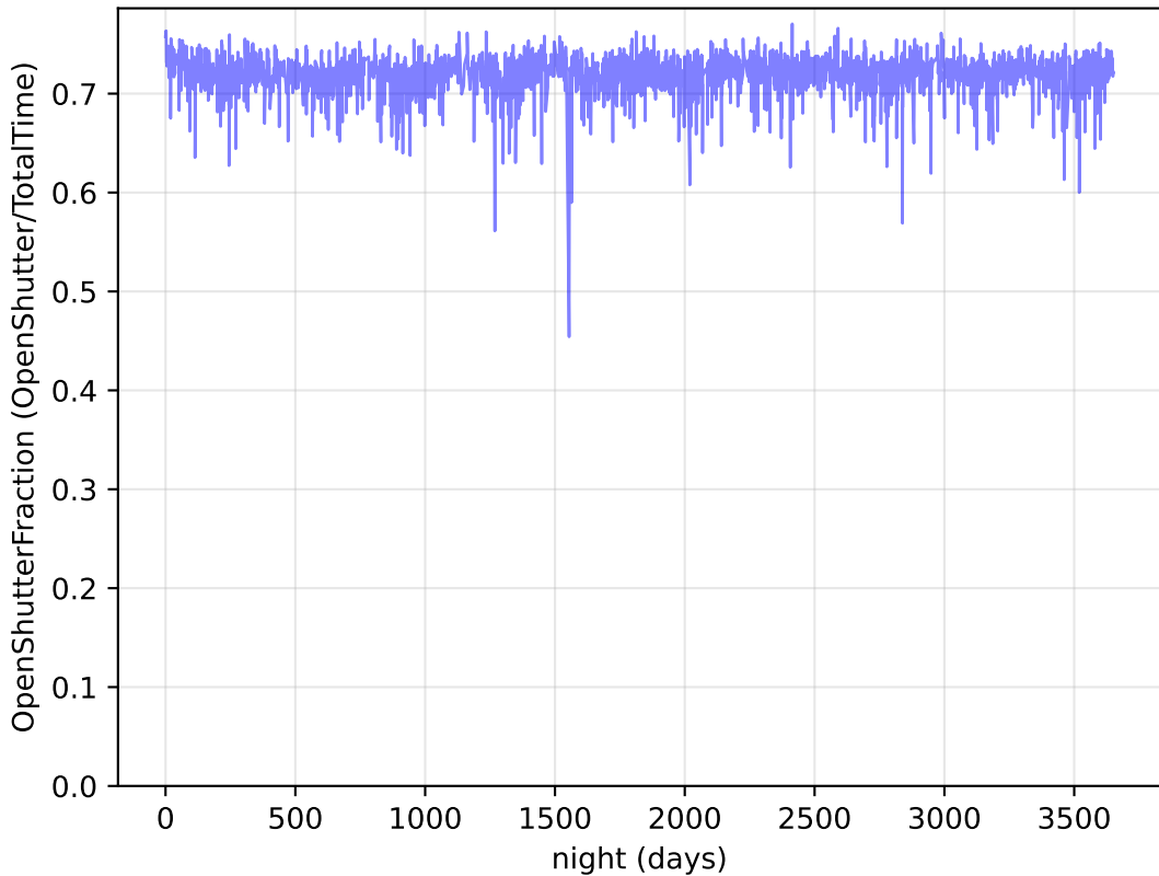
too_100_4v3.4_10yrs : OpenShutterFraction
