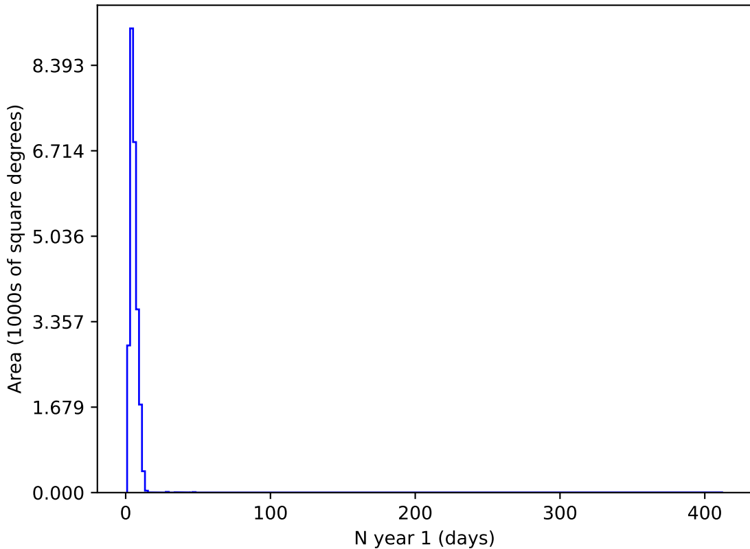
too_100_4v3.4_10yrs u and night < 365: N year 1
