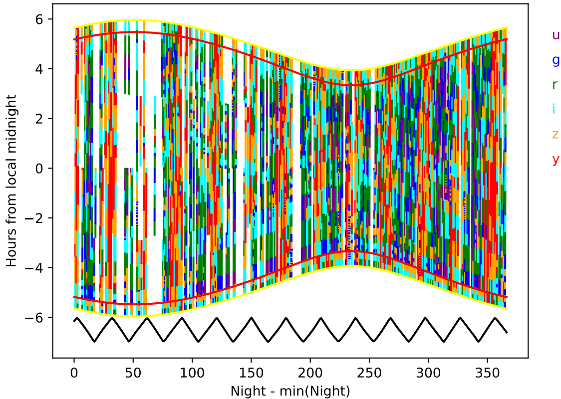
too_100_4v3.4_10yrs year 9-10: Hourglass
