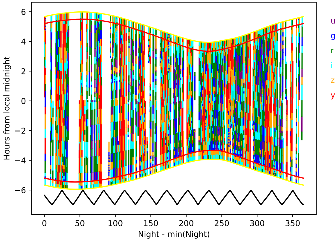
too_100_4v3.4_10yrs year 4-5: Hourglass
