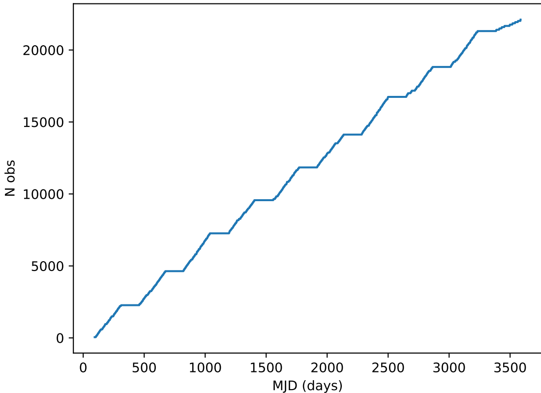
too_100_4v3.4_10yrs note like DD:ECDFS%: Cumulative
