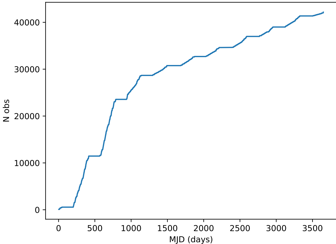
too_100_4v3.4_10yrs note like DD:COSMOS%: Cumulative
