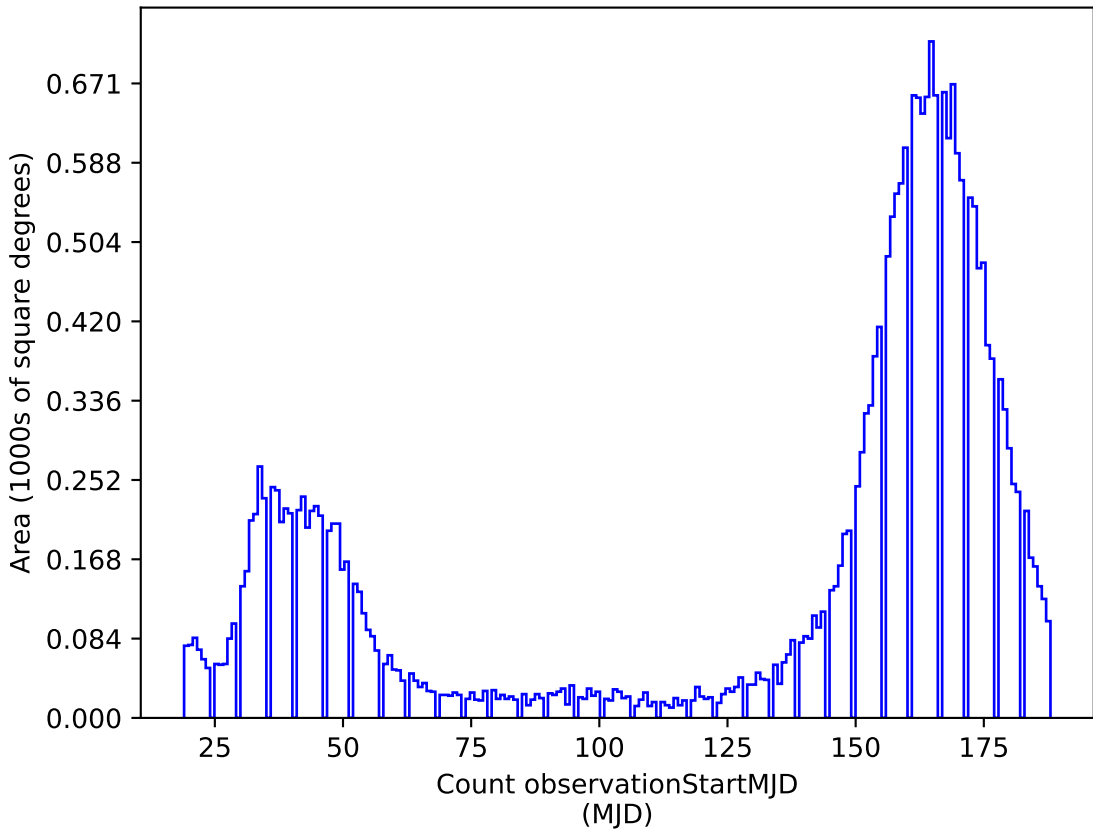
too_100_4v3.4_10yrs z: Count observationStartMJD
