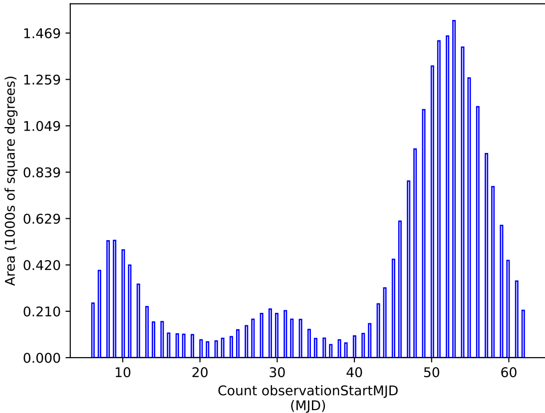
too_100_4v3.4_10yrs u: Count observationStartMJD
