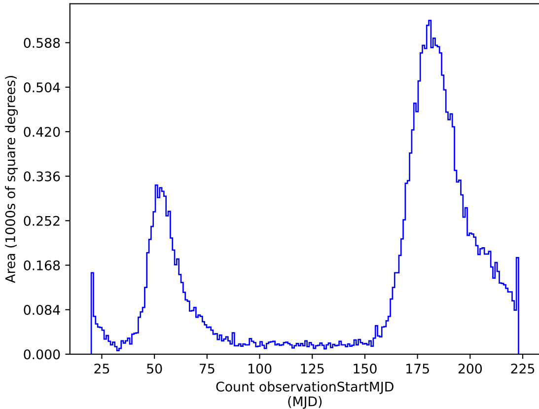
too_100_4v3.4_10yrs r: Count observationStartMJD
