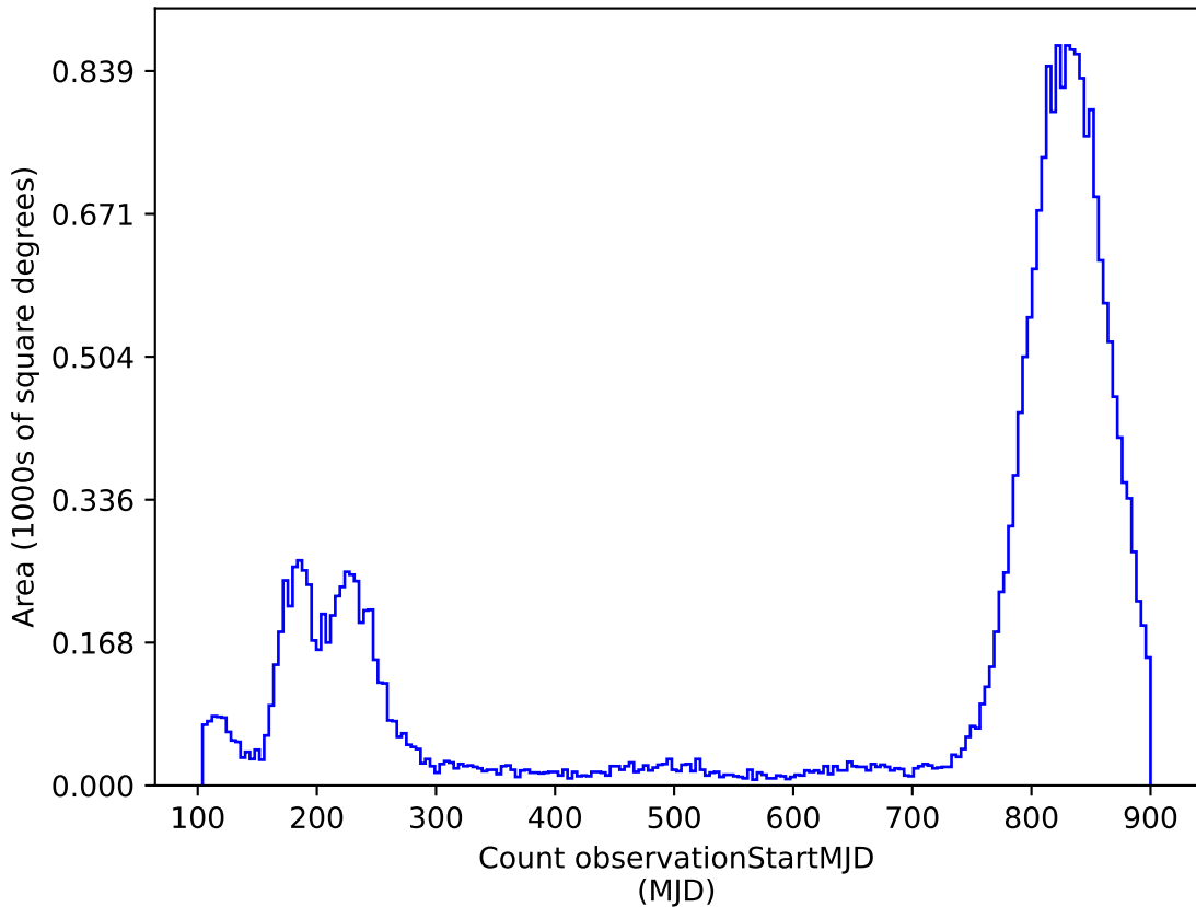
too_100_4v3.4_10yrs : Count observationStartMJD
