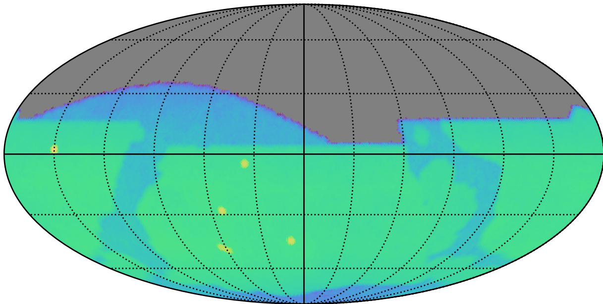
too_100_4v3.4_10yrs z: CoaddM5
