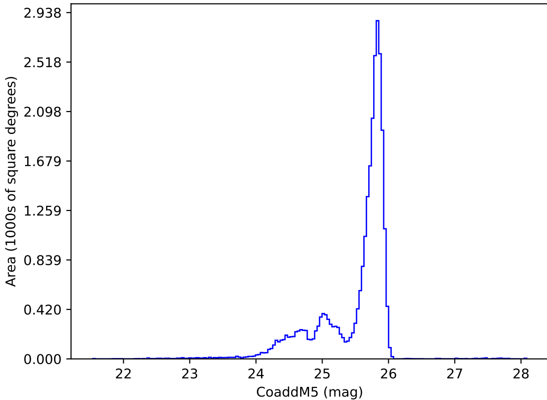
too_100_4v3.4_10yrs z: CoaddM5
