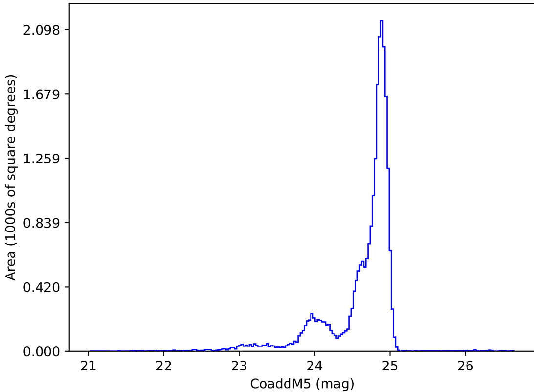
too_100_4v3.4_10yrs y: CoaddM5
