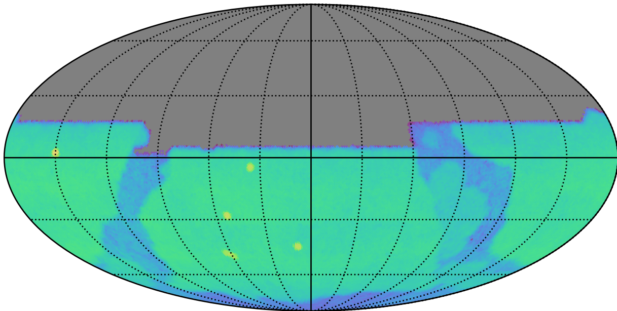
too_100_4v3.4_10yrs u: CoaddM5
