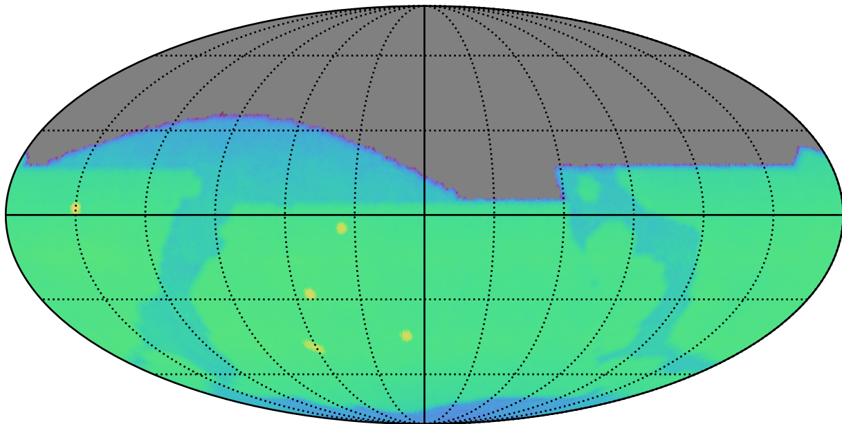
too_100_4v3.4_10yrs i: CoaddM5
