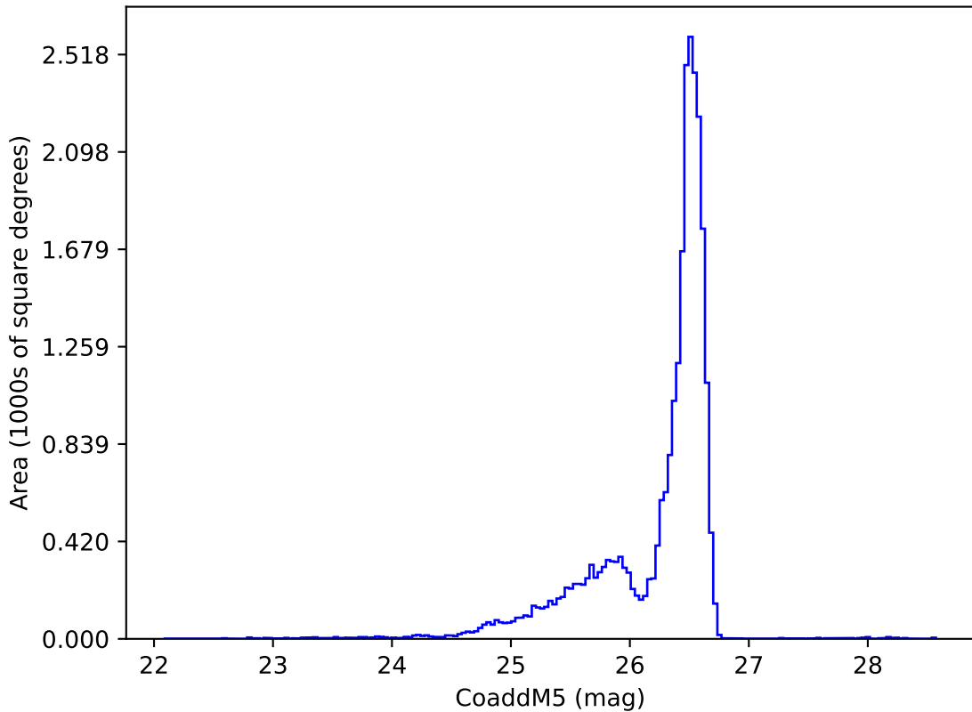
too_100_4v3.4_10yrs i: CoaddM5
