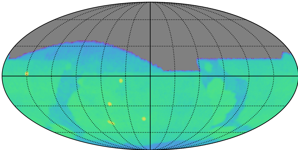
too_100_4v3.4_10yrs g: CoaddM5
