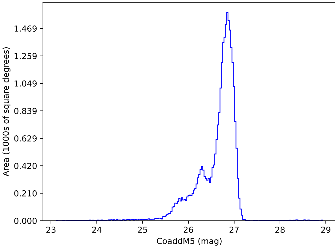
too_100_4v3.4_10yrs g: CoaddM5
