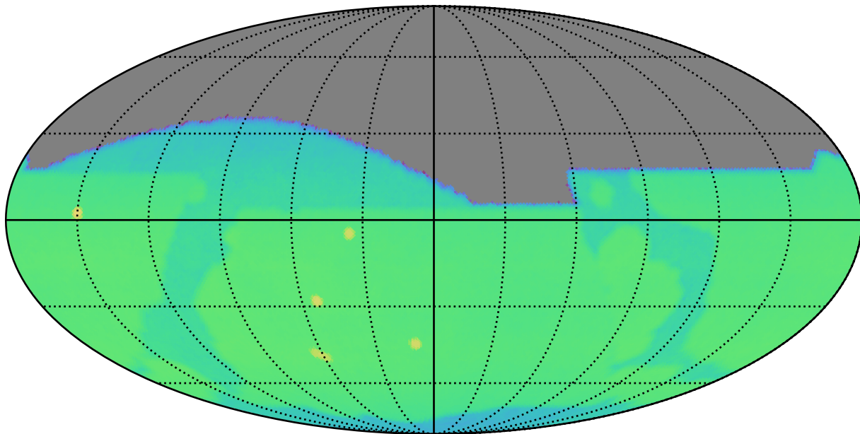
too_100_4v3.4_10yrs : CoaddM5
