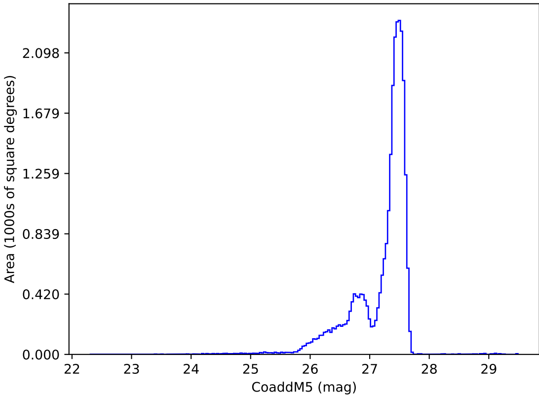
too_100_4v3.4_10yrs : CoaddM5
