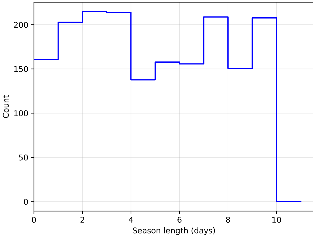
too_100_4v3.4_10yrs DD:WFD all bands: SeasonLength
