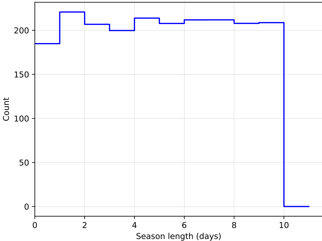
too_100_4v3.4_10yrs DD:ELAISS1 all bands: SeasonLength
