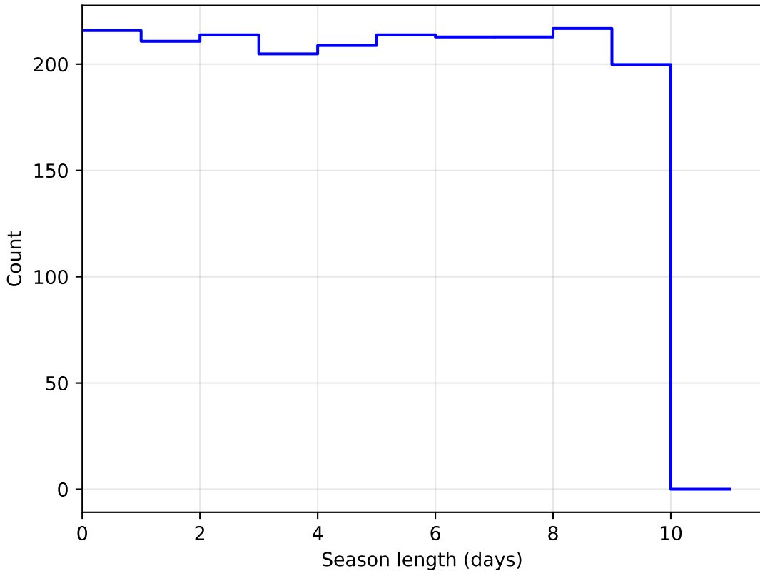
too_100_4v3.4_10yrs DD:ECDFS all bands: SeasonLength
