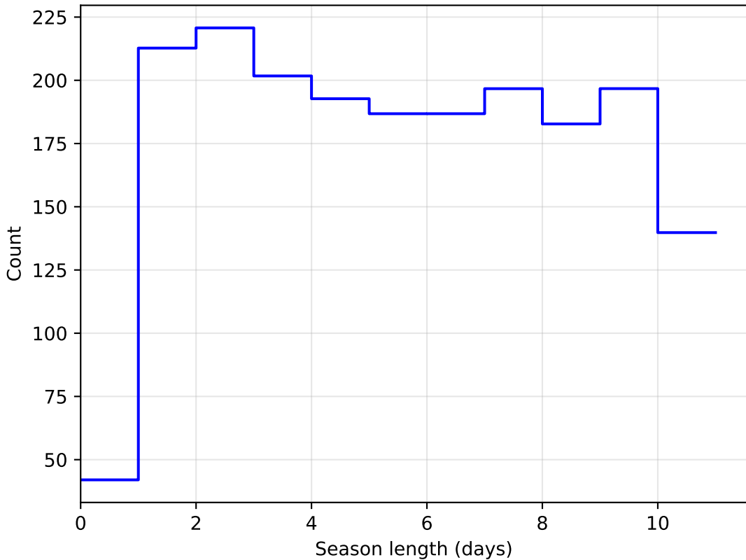
too_100_4v3.4_10yrs DD: COSMOS all bands: SeasonLength
