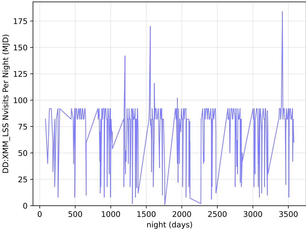
too_100_4v3.4_10yrs all bands: DD:XMM_LSS Nvisits Per Night
