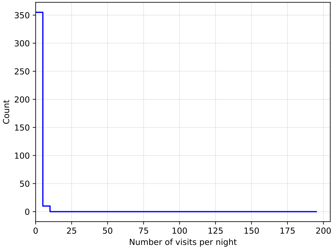
too_100_4v3.4_10yrs all bands: DD:WFD NVisitsPerNight
