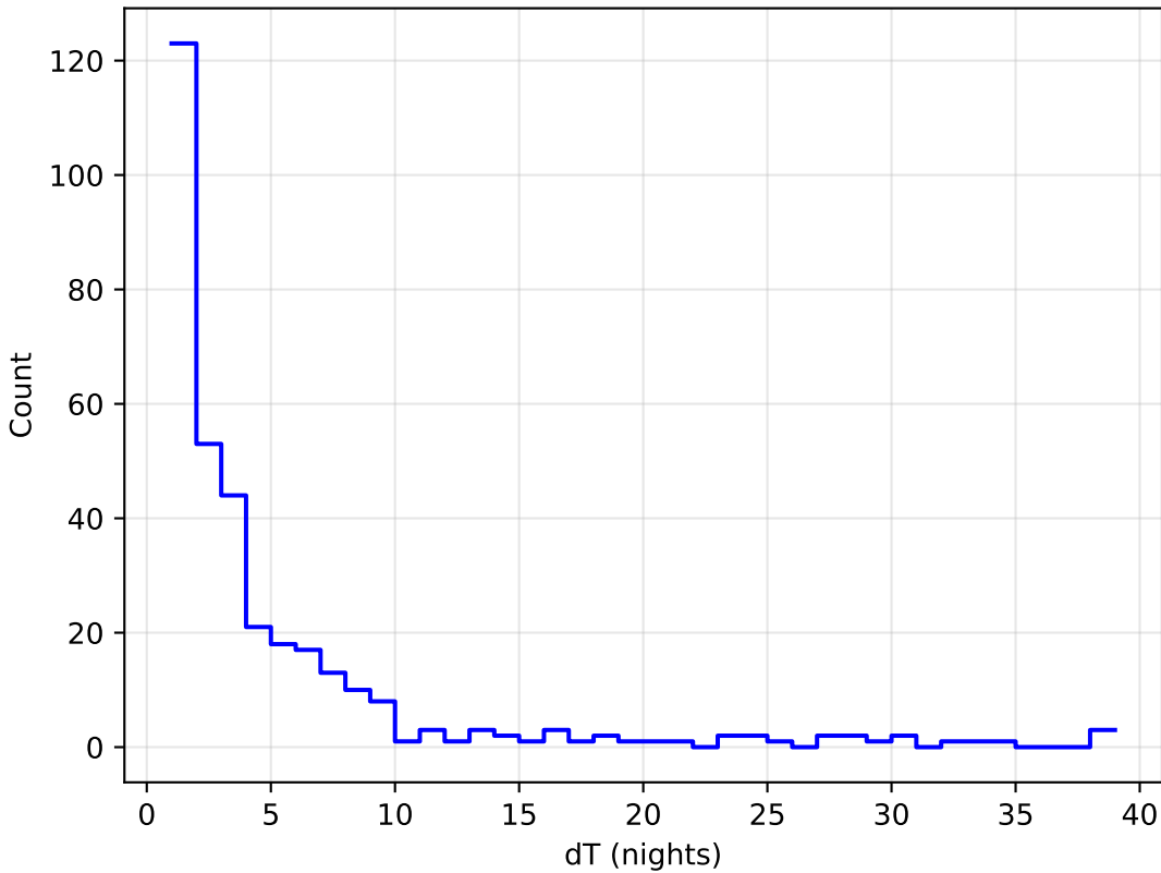
too_100_4v3.4_10yrs all bands: DD:WFD Delta Nights Histogram
