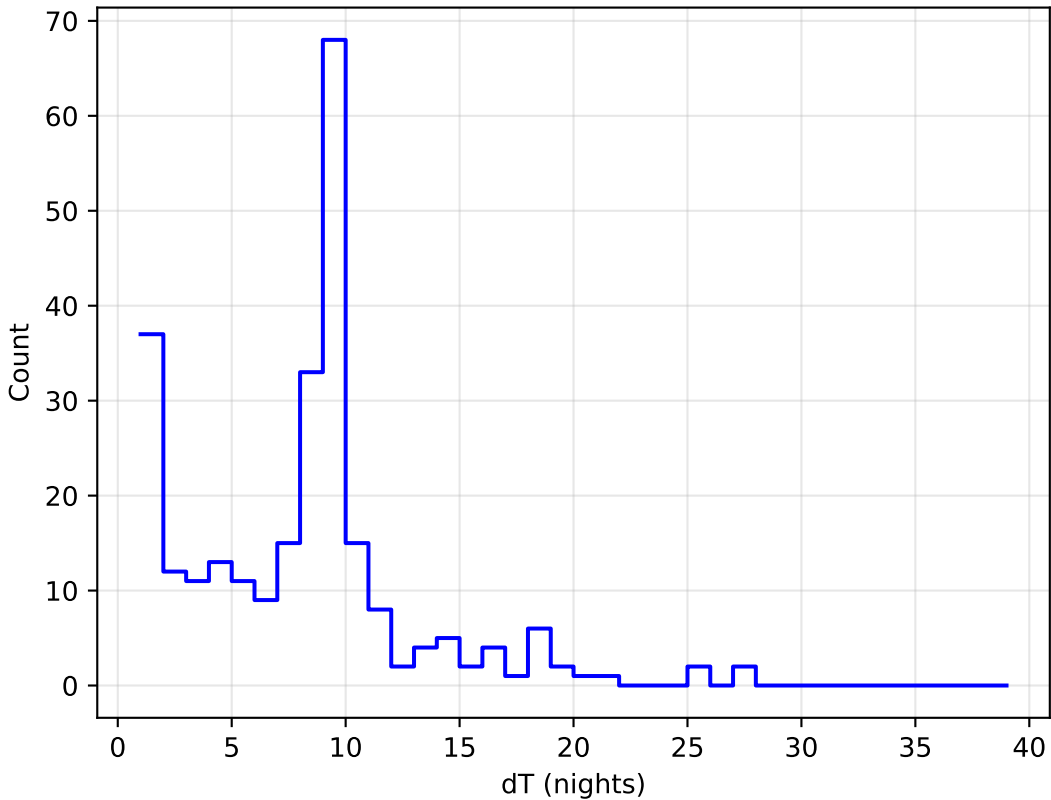
too_100_4v3.4_10yrs all bands: DD:ELAISS1 Delta Nights Histogram
