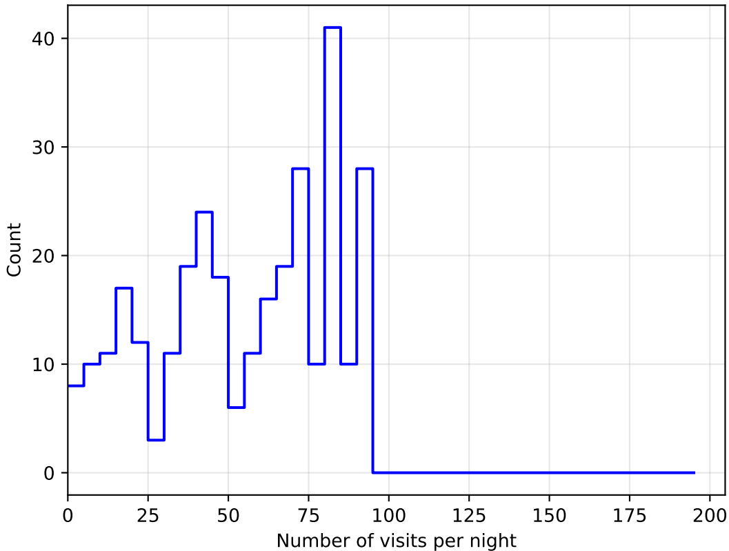
too_100_4v3.4_10yrs all bands: DD:EDFS NVisitsPerNight
