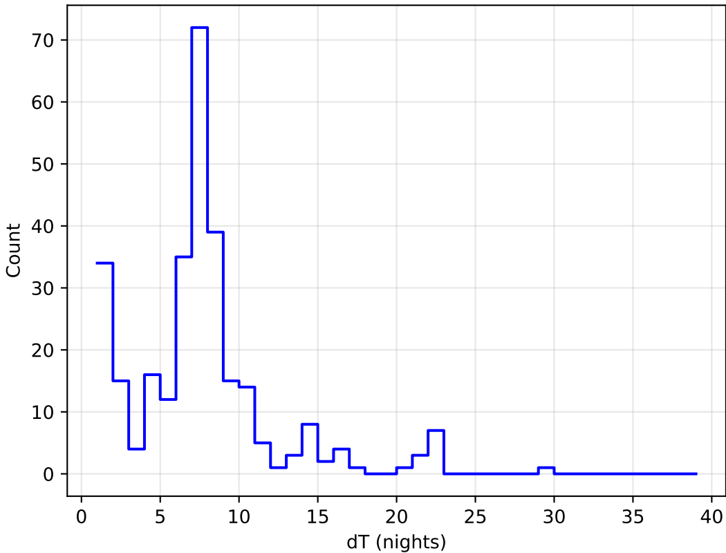
too_100_4v3.4_10yrs all bands: DD:EDFS Delta Nights Histogram
