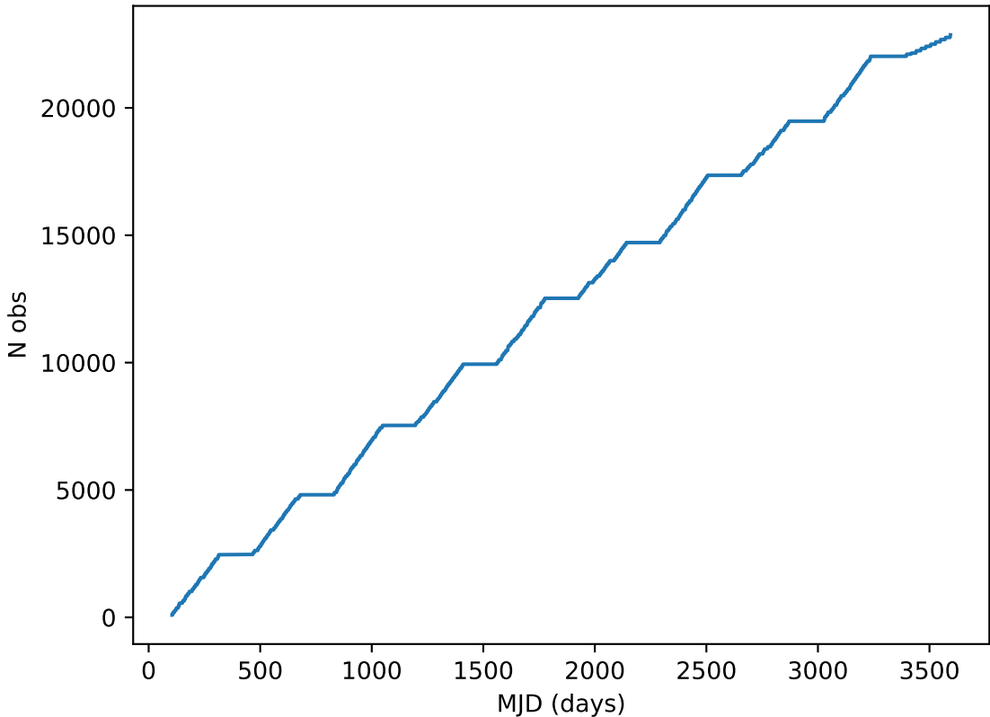
too_100_4v3.4_10yrs all bands: DD:EDFS Cumulative NVisits
