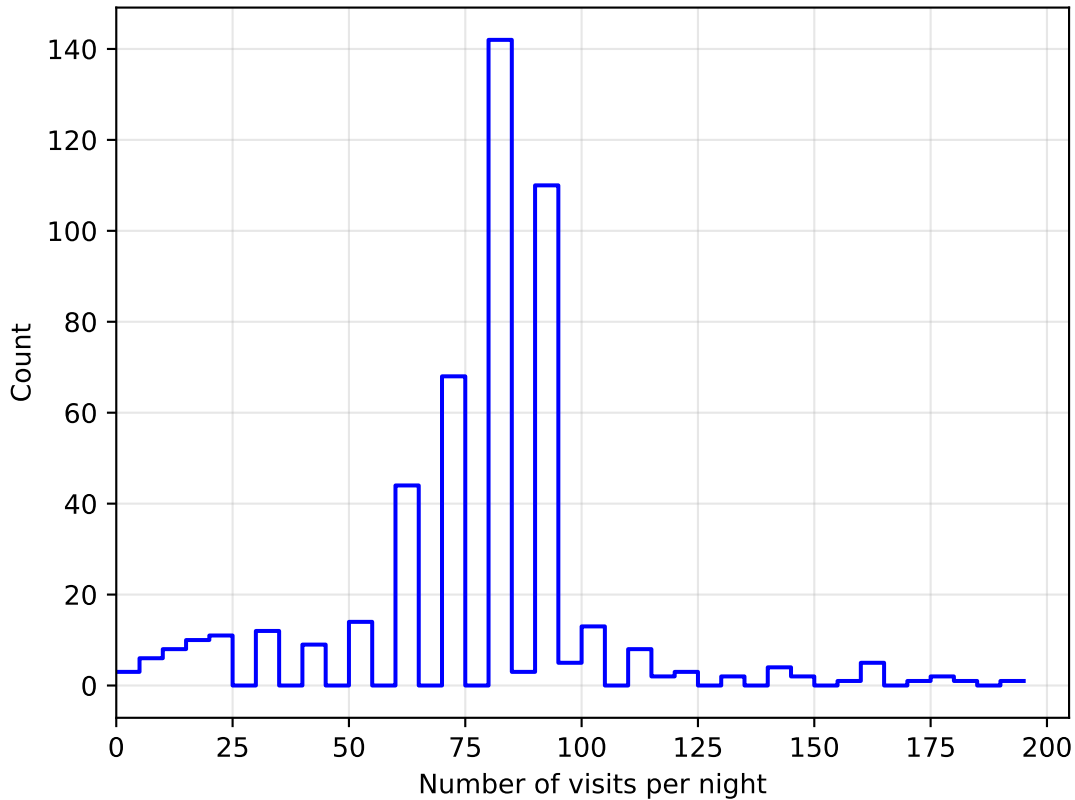
too_100_4v3.4_10yrs all bands: DD:COSMOS NVisitsPerNight
