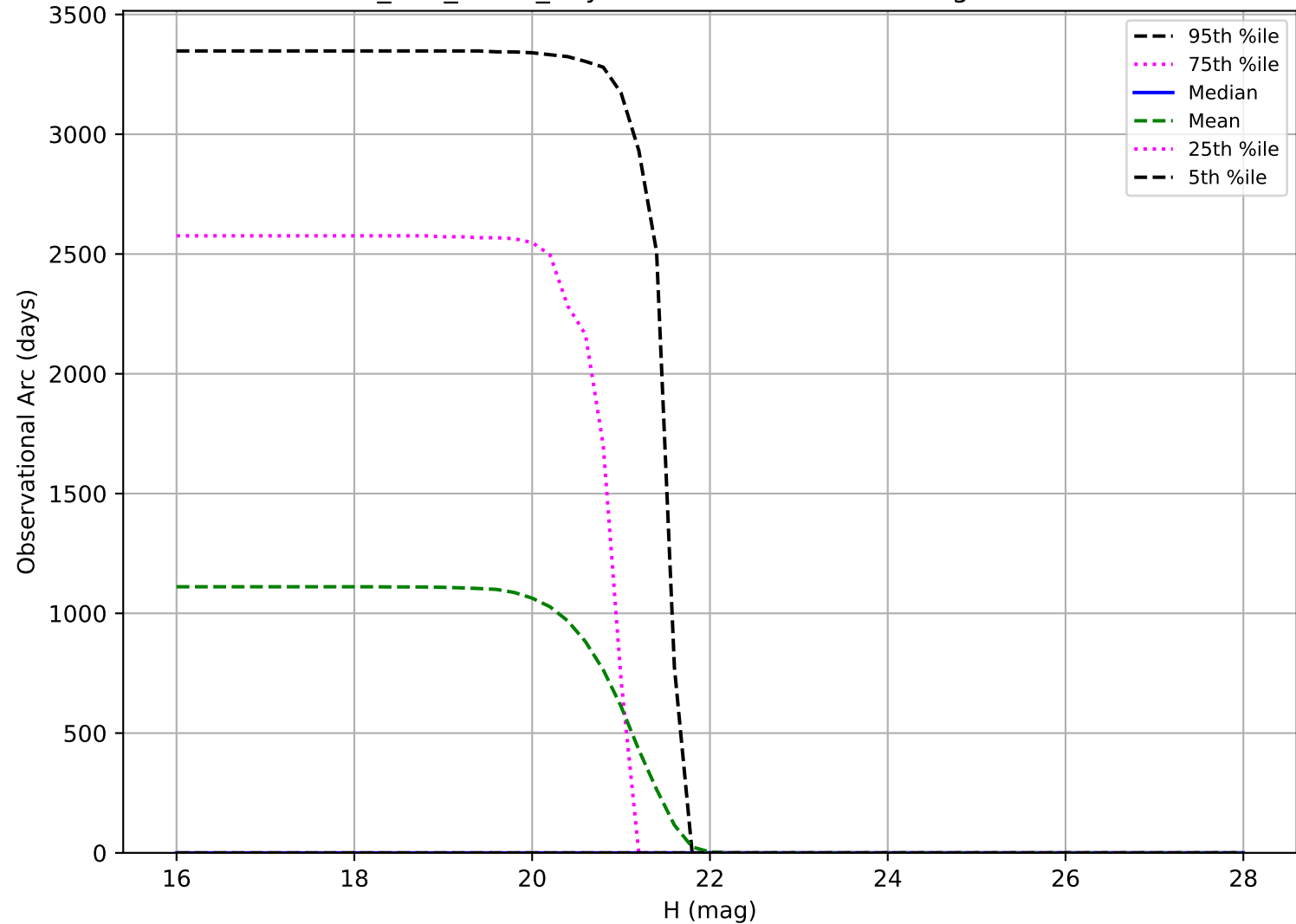
too_100_1v3.4_10yrs: Observational Arc Length Vatira
