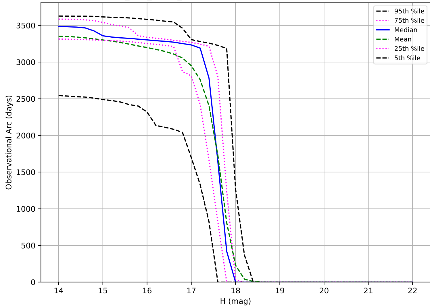
too_100_1v3.4_10yrs: Observational Arc Length Trojan
