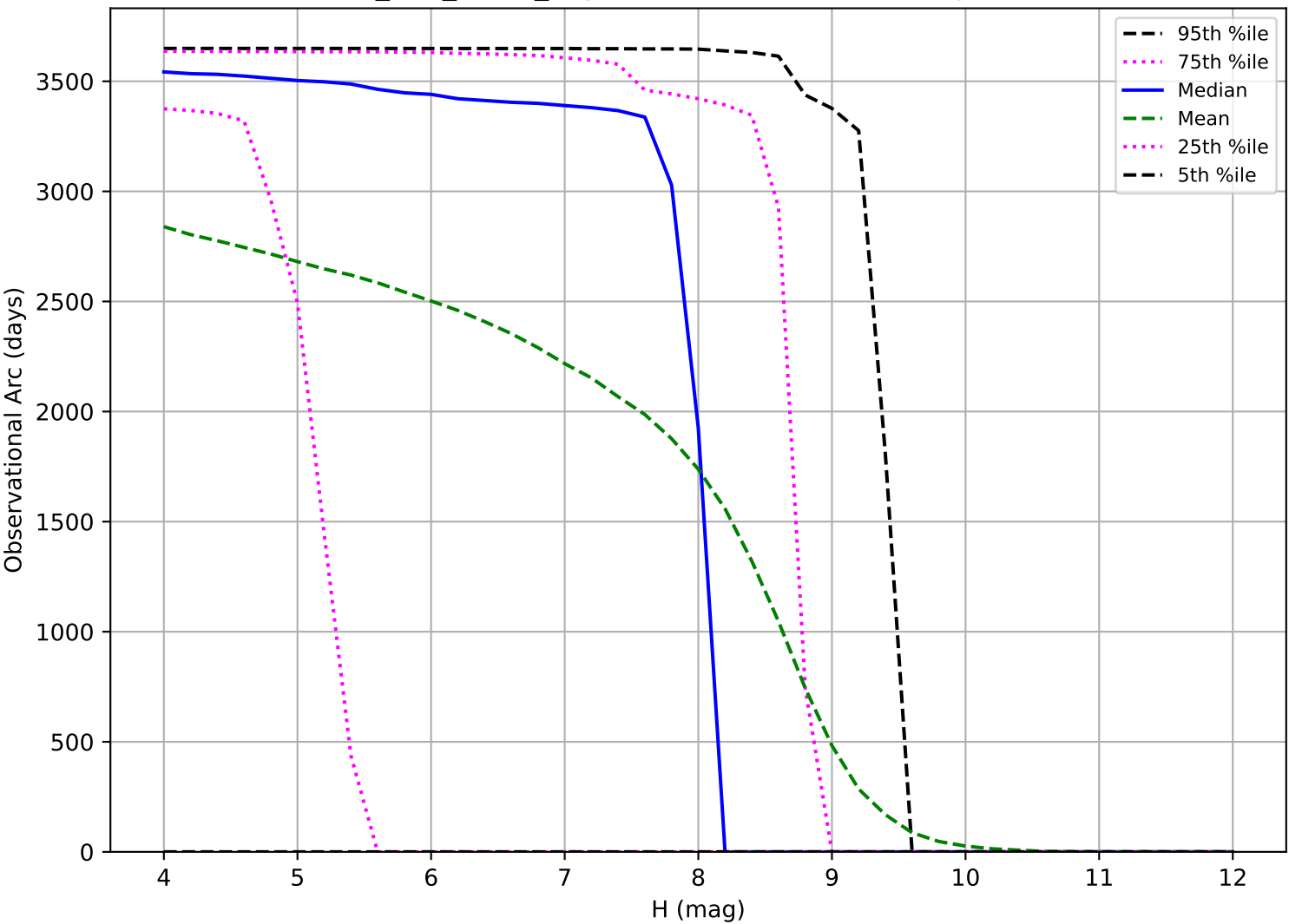
too_100_1v3.4_10yrs: Observational Arc Length TNO
