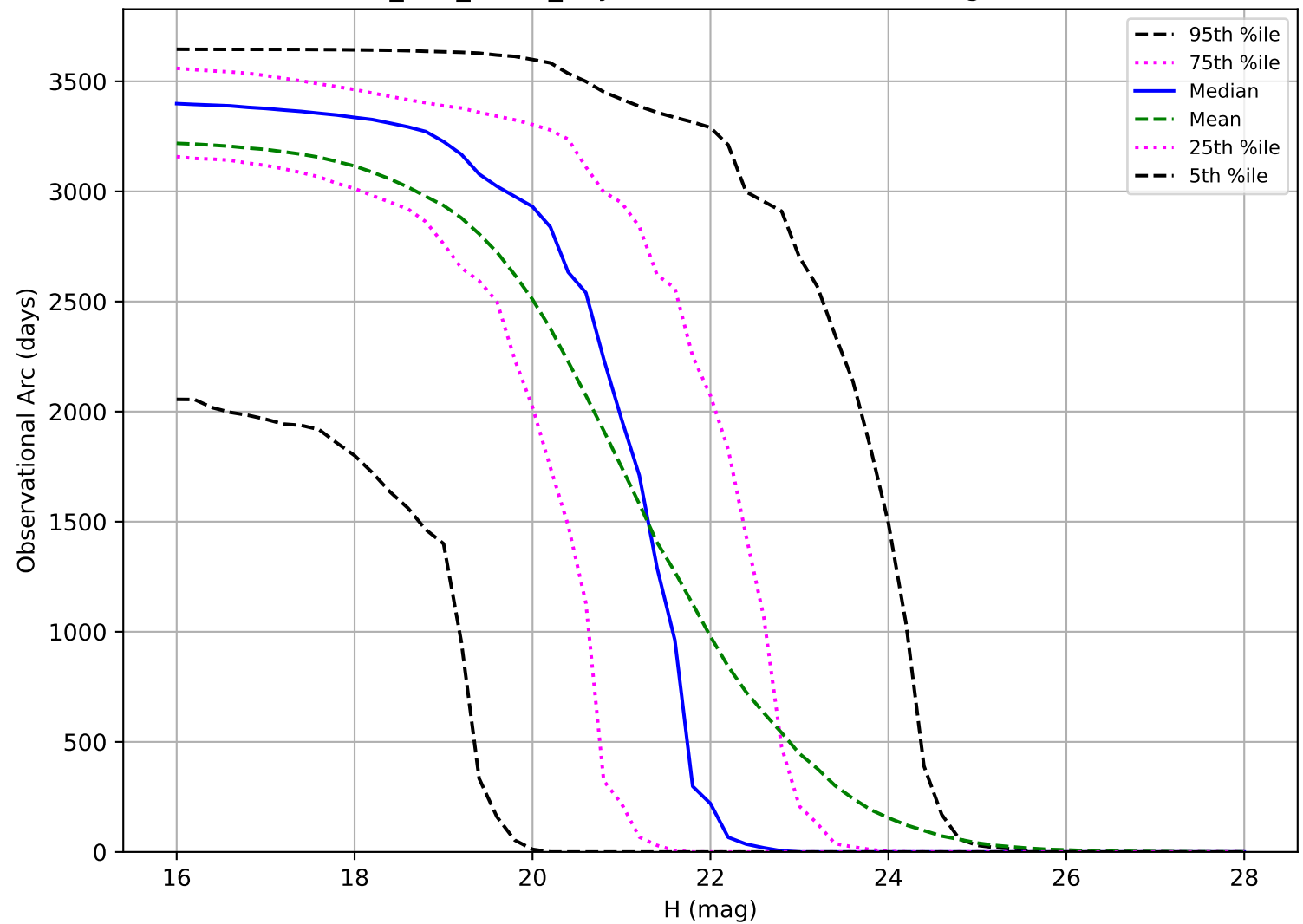
too_100_1v3.4_10yrs: Observational Arc Length PHA
