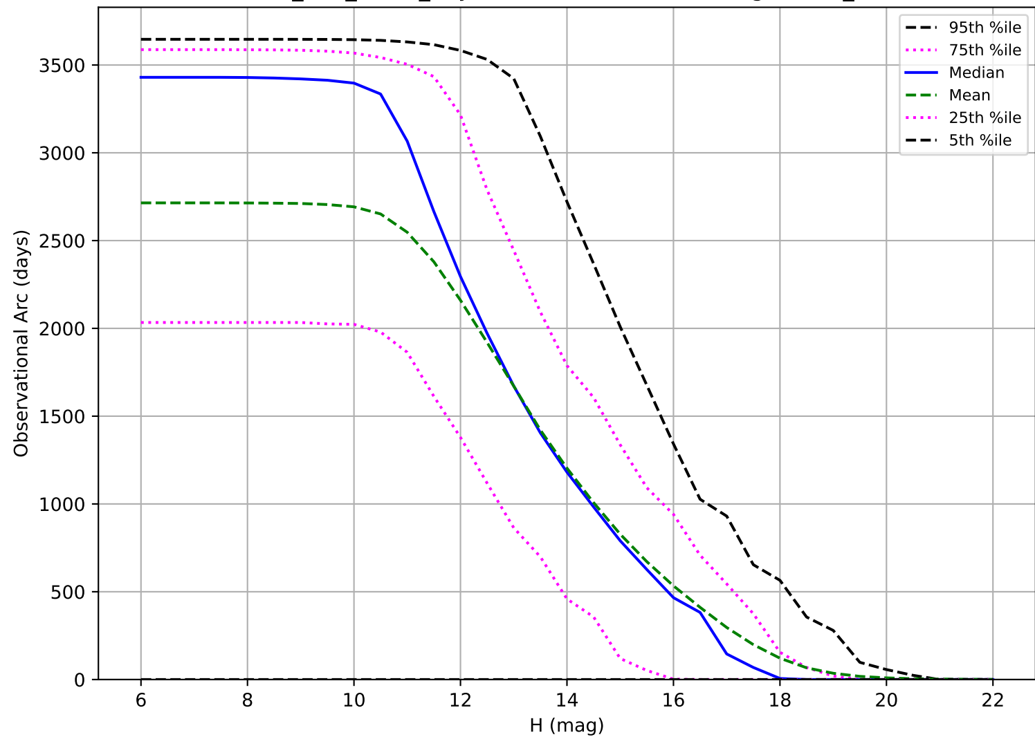
too_100_1v3.4_10yrs: Observational Arc Length OCC_r5
