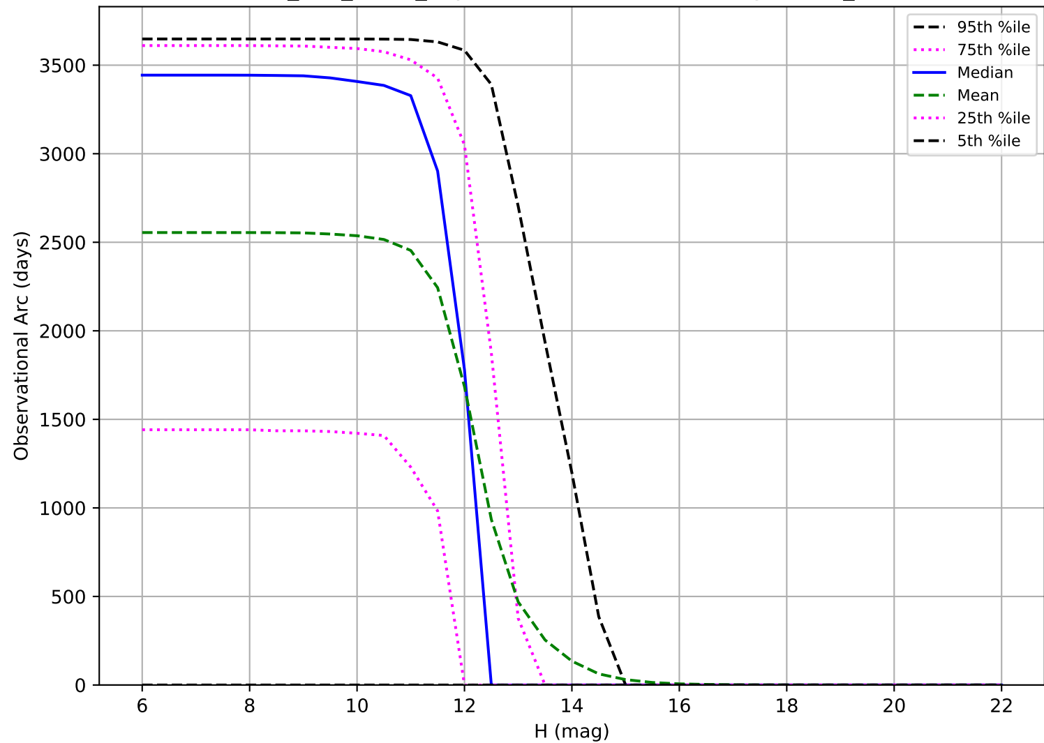
too_100_1v3.4_10yrs: Observational Arc Length OCC_r20
