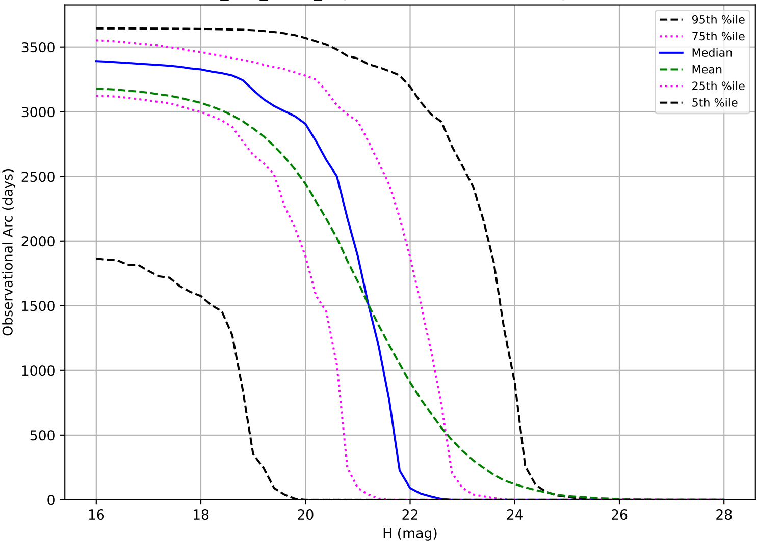
too_100_1v3.4_10yrs: Observational Arc Length NEO
