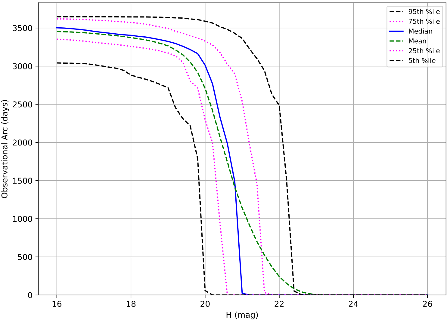
too_100_1v3.4_10yrs: Observational Arc Length MBA
