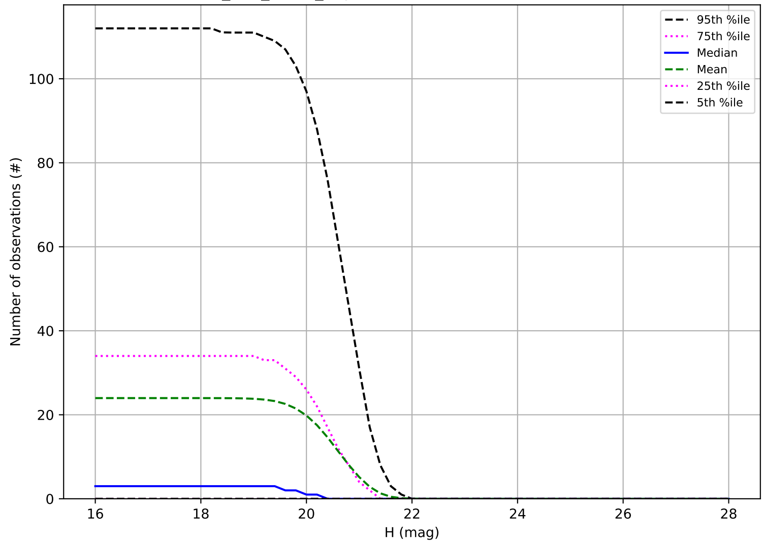
too_100_1v3.4_10yrs: Number of observations Vatira
