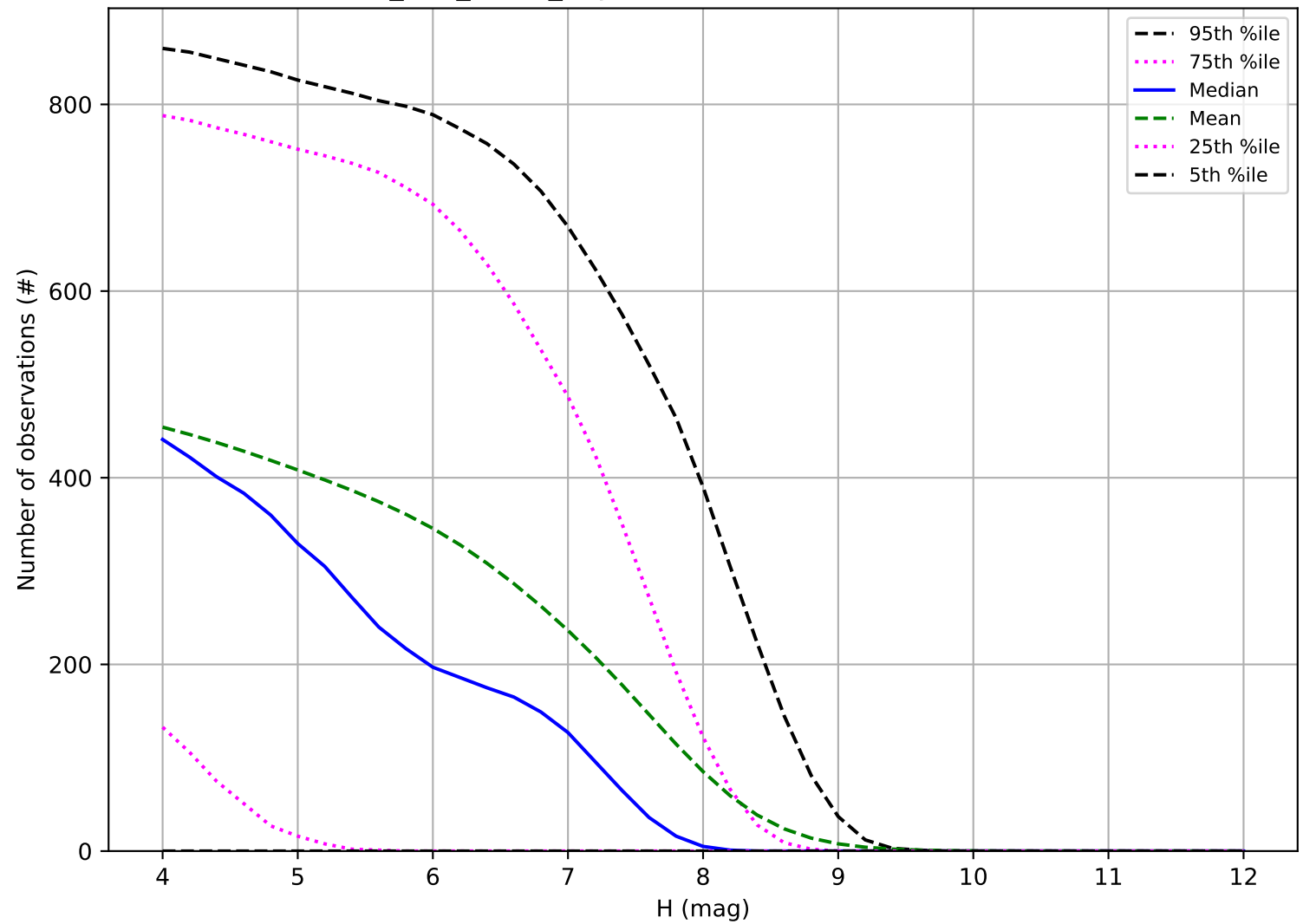
too_100_1v3.4_10yrs: Number of observations TNO
