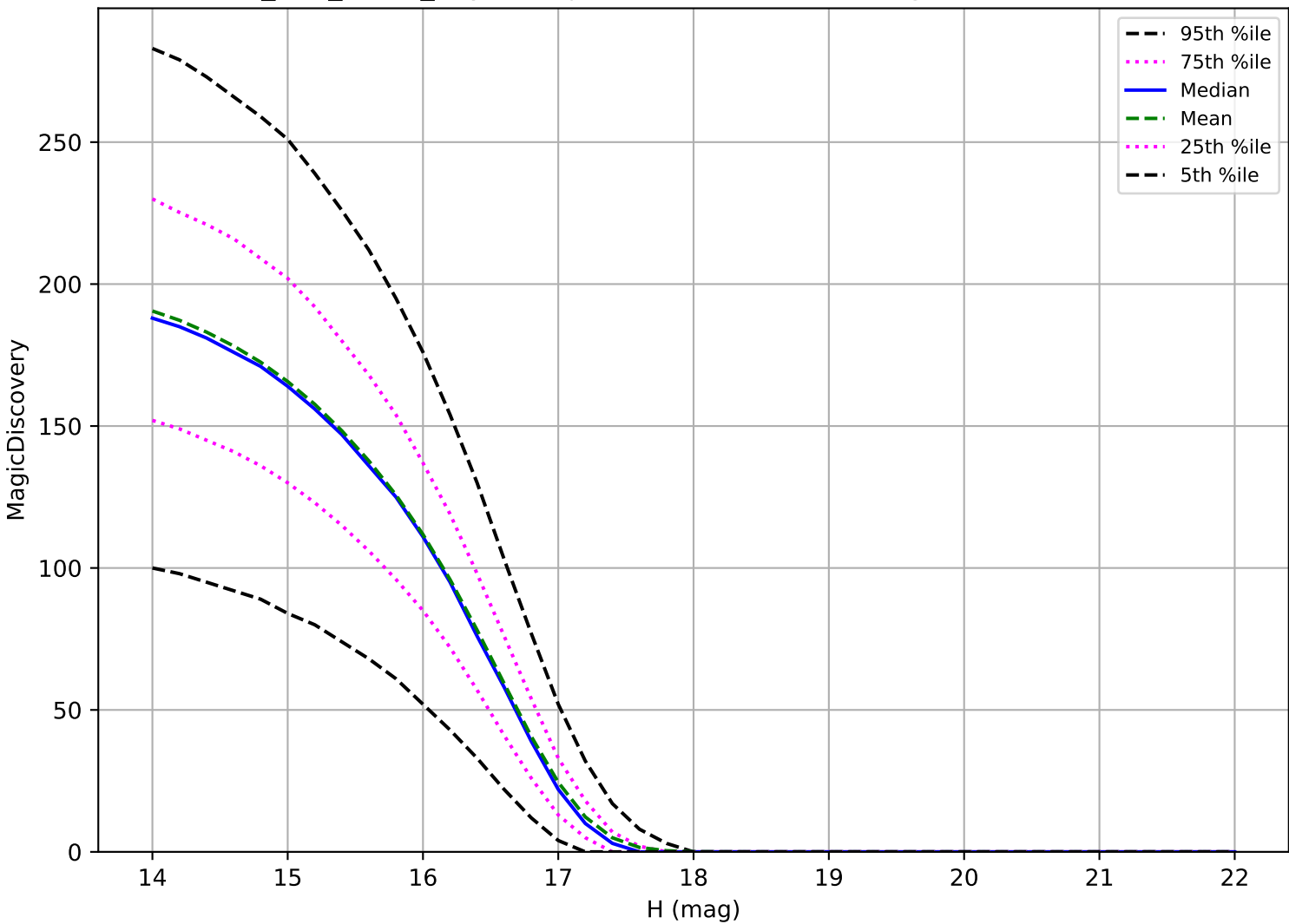
too_100_1v3.4_10yrs: Trojan 6 detections in 60 nights detection loss
